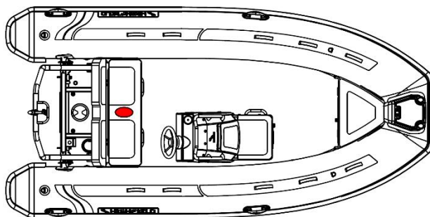
Location for portable extinguisher (CL420-460)
