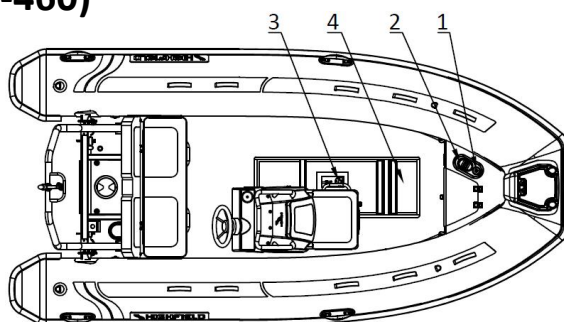
Chart of Fuel System
